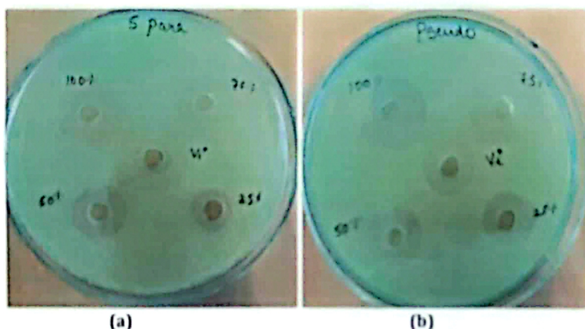
Figure 5: Antibacterial activity of vinegar (acetic acid) against a) Salmonella paratyphi & b) Pseudomonas aeruginosa
