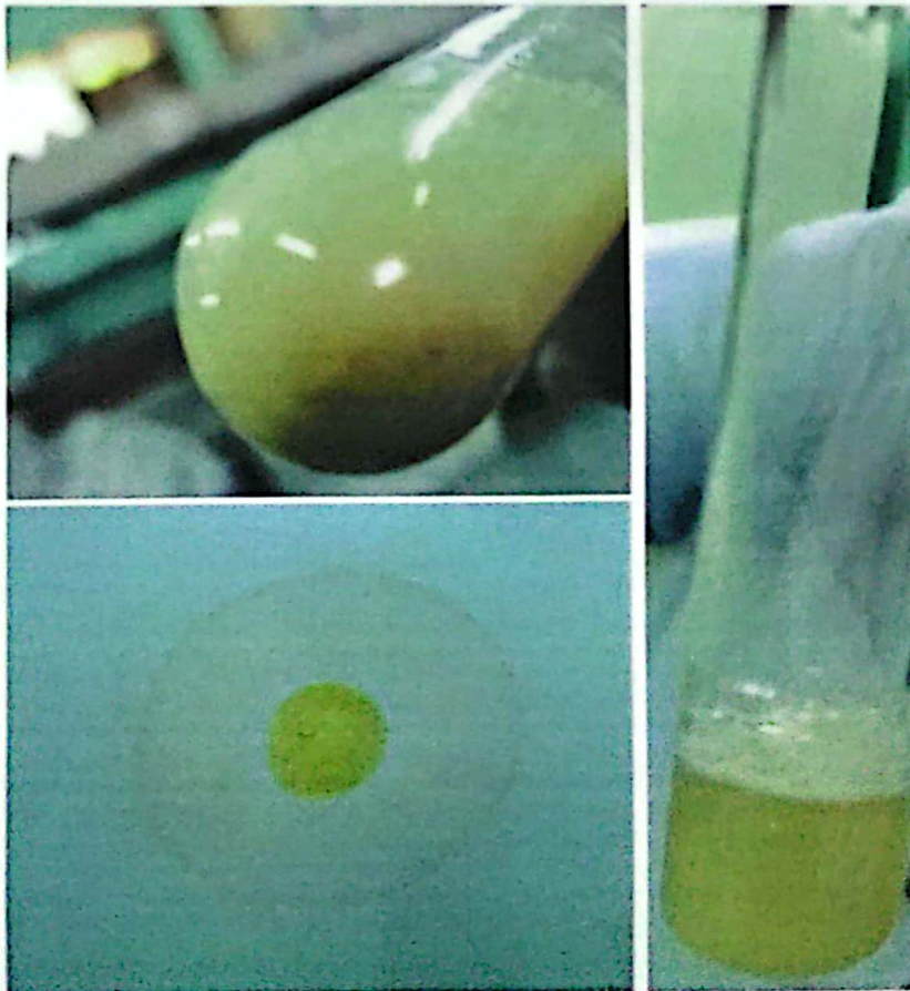
Figure 3: Alcohol production by Iodoform test and Qualitative test for acetic acid (presence of effervescence)
