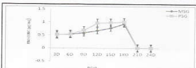
Fig. 2. Total RNA concentration in MSG and PSG
