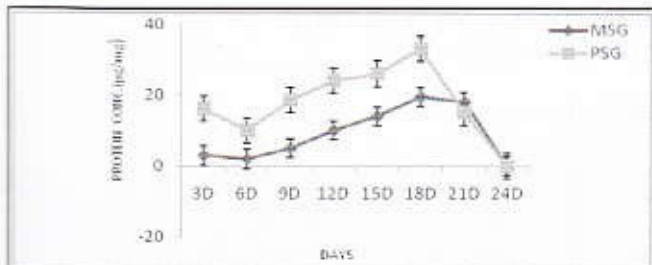
Fig. 3. Total protein concentration in MSG and PSG
