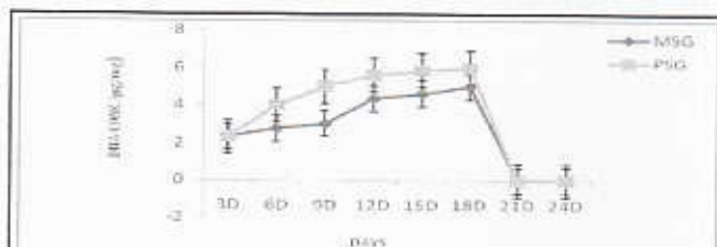
Fig. 1. Total DNA concentration in MSG and PSG
