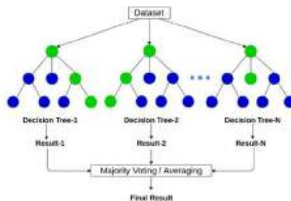
Figure 6: Random Forest.
