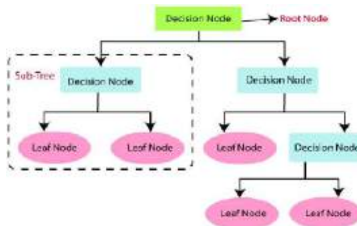
Figure 5: Decision Tree.
