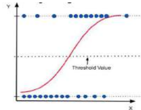
Figure 3: Logistic Regression.
