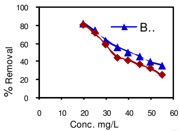
Figure. 3- Effect of Contact time on removal of Pb(II)
