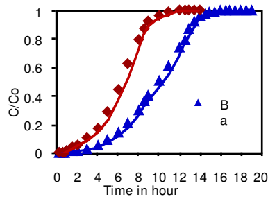
Figure. 6- Breakthrough curve for Pb(II)
