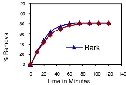
Figure. 2- Effect of Contact time on removal of Pb(II)
