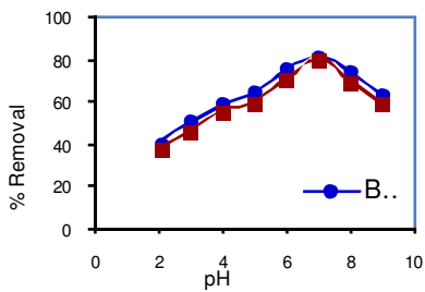
Figure.1- Effect of pH on removal of Pb(II)
