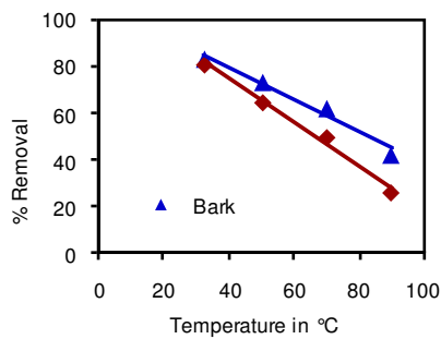
Figure. 5- Effect of Temperature on removal of Pb(II)
