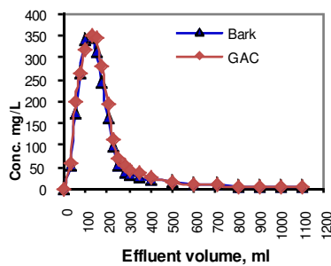
Figure. 6- Breakthrough curve for Pb(II)
