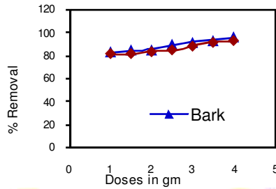
Figure. 4- Effect of Doses on removal of Pb(II)
